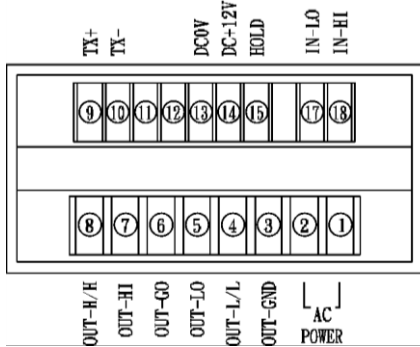
* RS-485 & 5-TRANSMITTER OUTPUT:
